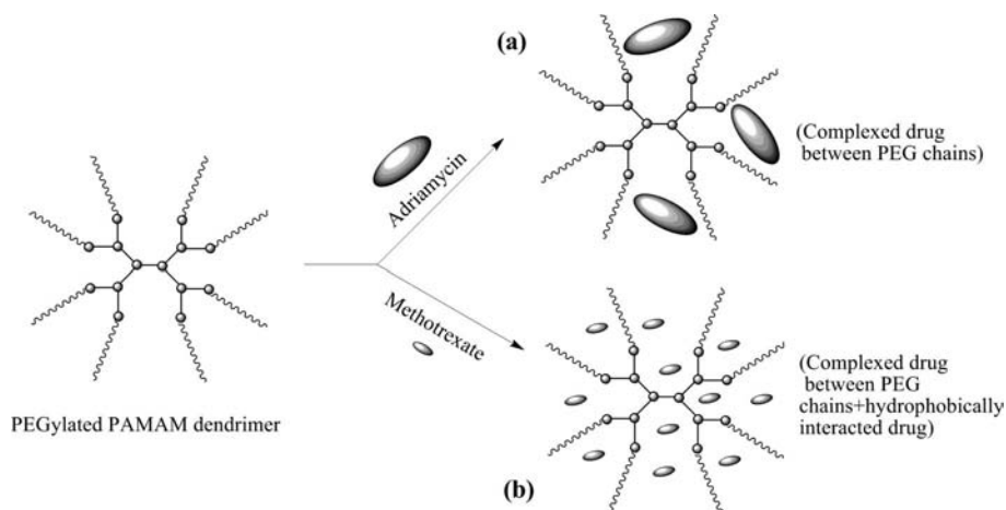
Figure 10. Schematic diagram showing drug loading in PEGylated dendrimers: (a) due to complexation of drug between PEG chains of dendrimer; (b) both due to existence of hydrophobic interaction owing to high acid–base feedback between drug and dendrimer as well as drug complexation between PEG chains of dendrimer.
